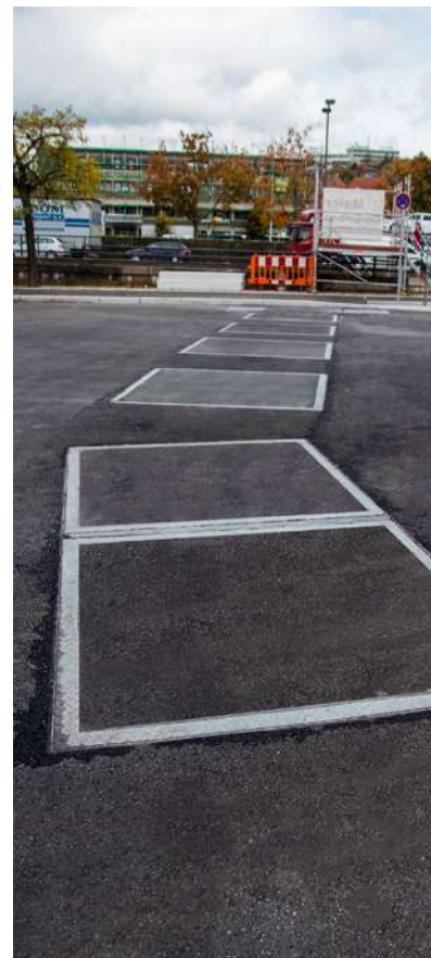
Backwater-proof covers filled with asphalt – Ansbach
