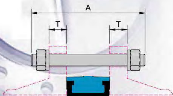
VF-730 WAFER TYPE 1.5" to 36.0"
