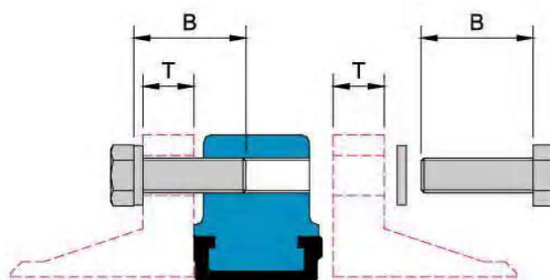
VF-733 FULL LUG TYPE 1.5" to 24.0"
